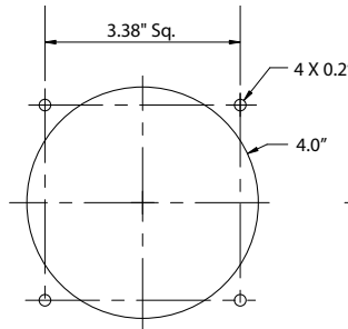
ANSI Mounting
